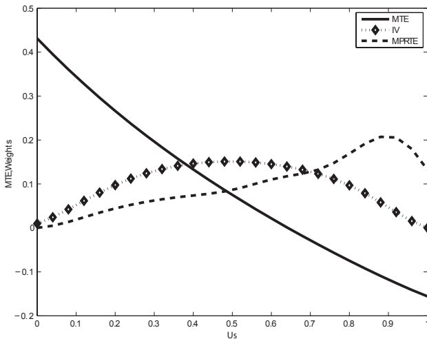
Figure 6: Weights for IV and MP RTE
