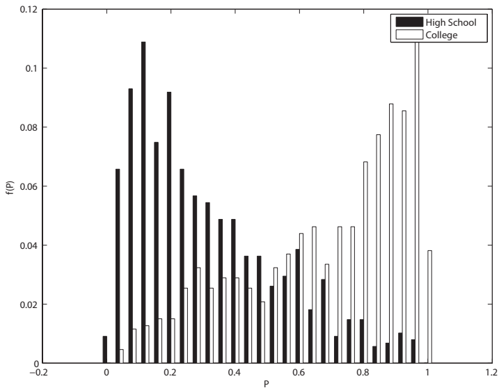
Figure 3: Support of P for S = 0 and S = 1
