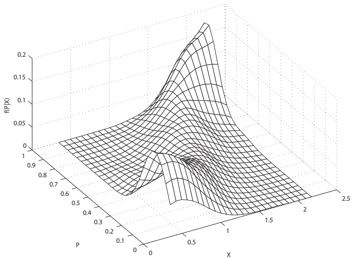
Figure 2: Support of P conditional on X
